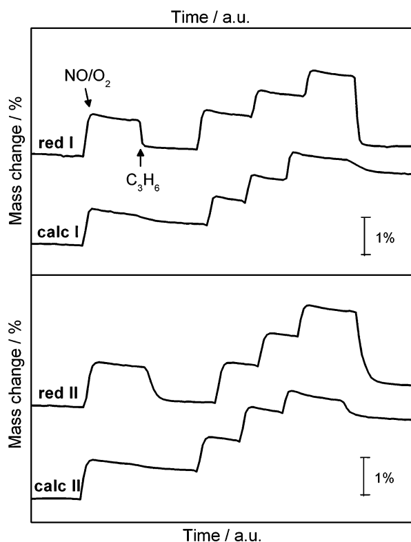
Fig. 7 Mass changes of the 0.74-Pt/Ba/CeO 2 catalyst resulting after one or three NO x storage cycles (mass uptake due to NO/O 2 pulses) and reduction with 1 ml of C 3 H 6 (mass loss) at 300 °C after calcinations at 700 °C (calc) and reduction at 400 °C with 4 ml H 2 . The upper part of the figure presents the NSR activity of the catalyst after one (I), the bottom part after two (II) perovskite formation-reduction cycles
